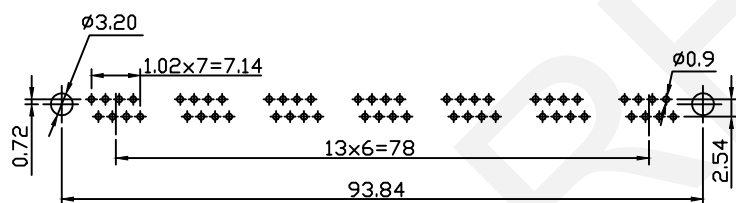
PCB Layout
