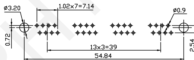
PCB Layout
