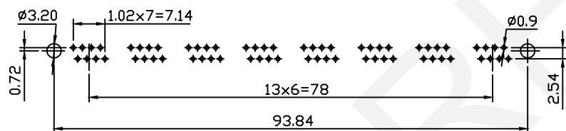
PCB Layout
