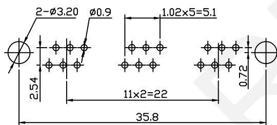
PCB Layout
