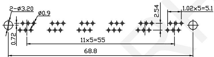
PCB Layout
