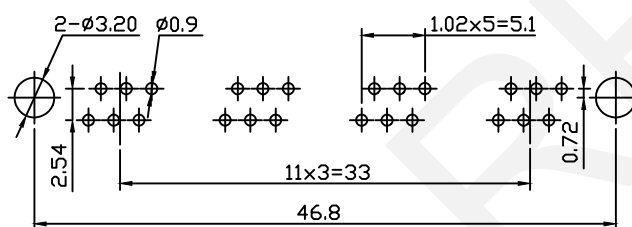
PCB Layout
