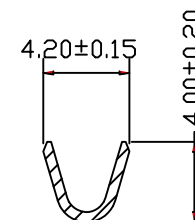
SECTION C-C
