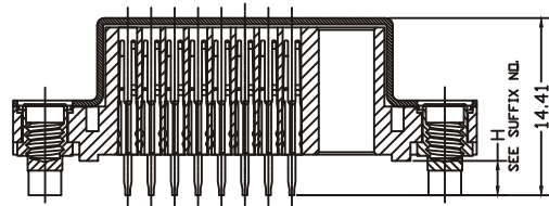
B-B SECTION
