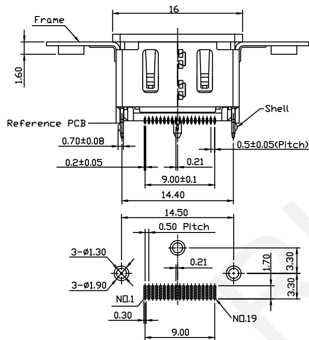
RECOMMENDED PCB LAYOUT (THICKNESS=1.6mm Tolerance±0.15mm)
