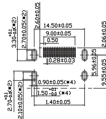
RECOMMENDED PCB LAYOUT (THICKNESS=1.6±0.15mm)
