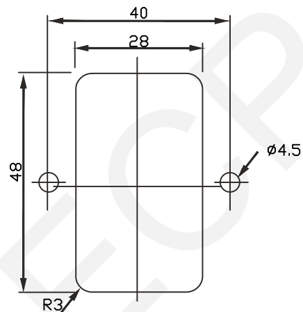
PANEL CUT-OUT
