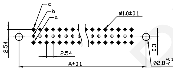
RECOMMENDED P.C.B LAYOUT(TOP VIEW) TOLERANCES:±0.10mm
