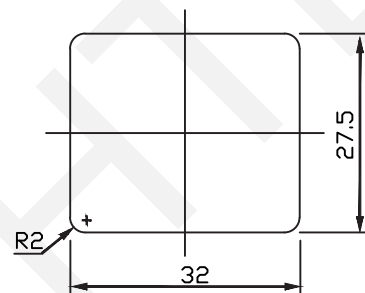
PANEL CUT-OUT
