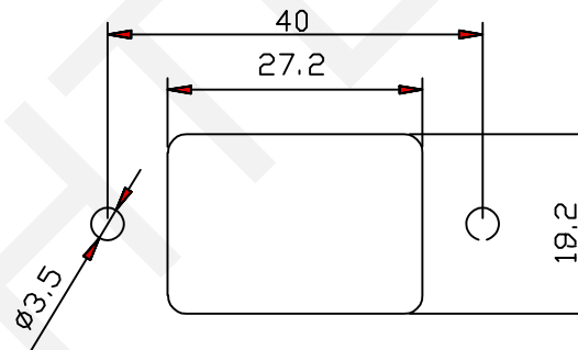
PANEL CUT-OUT
