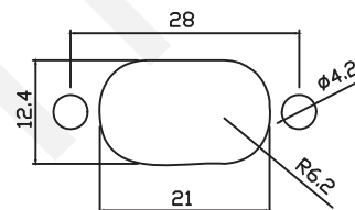
PANEL CUT-OUT
