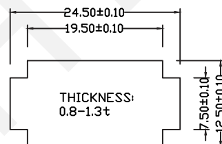
PANEL CUT-OUT
