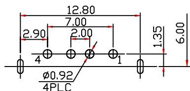
RECOMMENDED PCB LAYOUT TOLERANCE:±0.05mm
