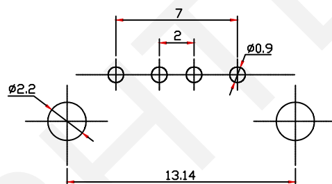
RECOMMENDED PCB LAYOUT TOLERANCE:±0.05mm
