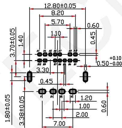
RECOMMENDED PCB LAYOUT GENERAL TOLERANCE: ±0.05
