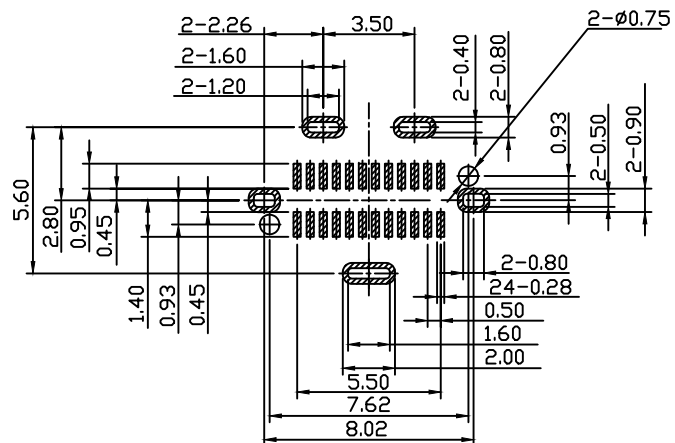
Recommended PCB Layout Tolerance: \pm 0.05\text{mm} , T=0.8\pm 0.10
