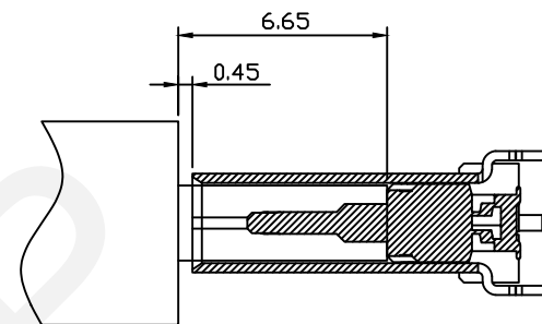
AFTER MATING
