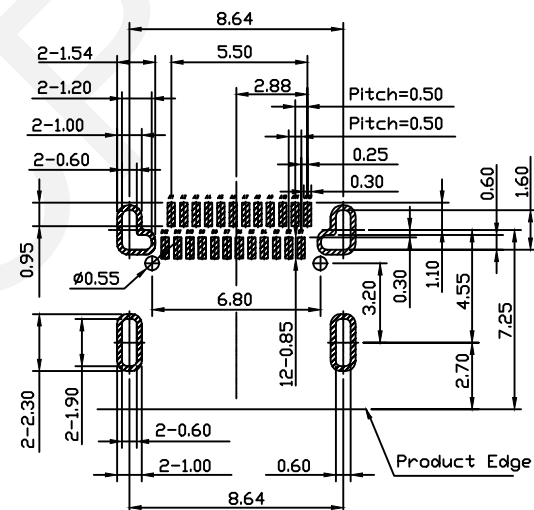
RECOMMENDED P.C.B.LAYOUT (TOP VIEW) TOLERANCE UNSPECIFIED \pm 0.05\text{mm}
