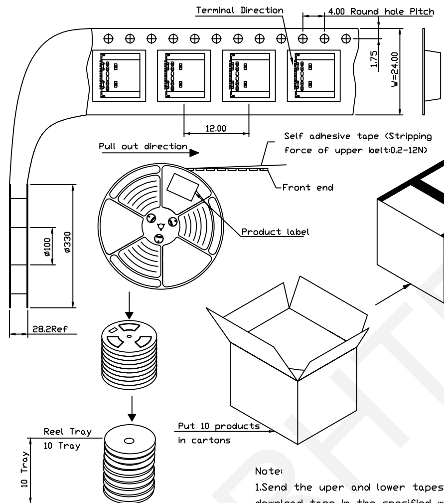
Packaging diagram:
