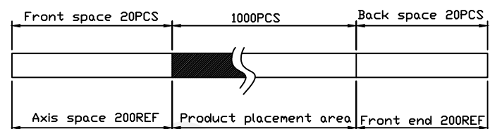
Packaging diagram:
