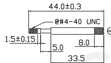
Long screw
