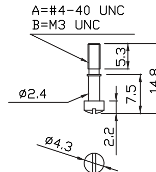
Short screw
