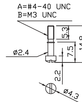
Short screw
