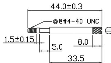
Long screw
