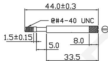
Long screw
