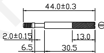
Long Screw
