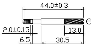
Long Screw
