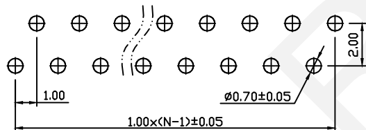
PCB LAYOUT
