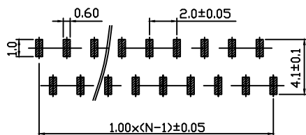
PCB LAYOUT
