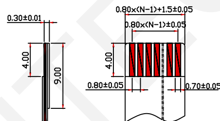
Recommended FPC Dimension
