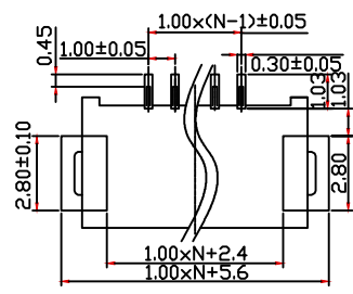
PCB Layout
