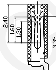
Section Y-Y
