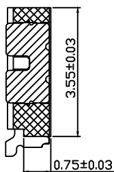
Section X-X
