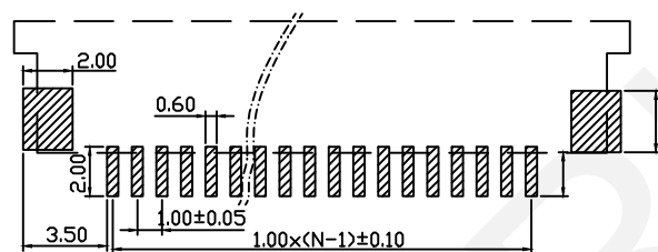
PCB Layout
