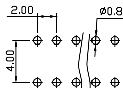
Recommended P.C.B Hole Layout
