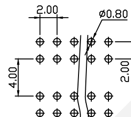
Recommended P.C.B Hole Layout
