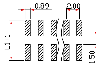
Recommended P.C.B Hole Layout
