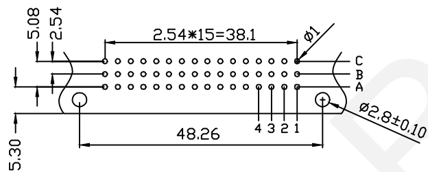
P.C.B card Layout
