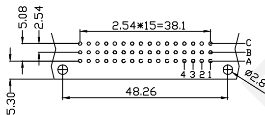
P.C.Bcard Layout
