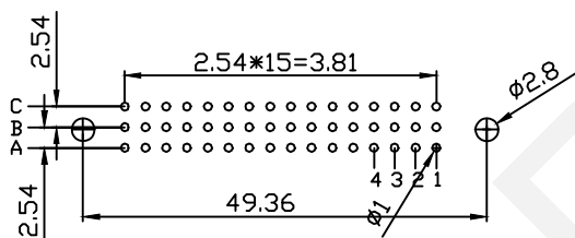
P.C.B card Layout
