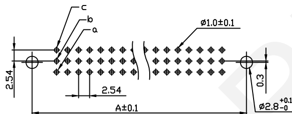
RECOMMENDED P.C.B LAYOUT(TOP VIEW) TOLERANCES:±0.10mm
