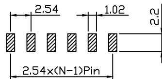
Recommended P.C.B Layout(Top Side) (PCB BOARD TOLERANCE±0.05)
