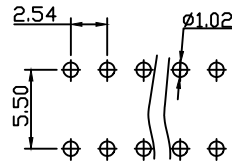
Recommended P.C.B Hole Layout
