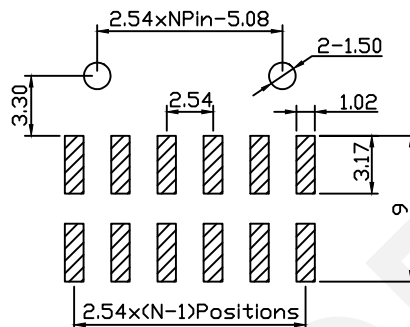
Recommended P.C.B Layout(Top VIEW) (PCB BOARD TOLERANCE±0.05)
