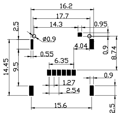
RECOMMENDED PCB LAYOUT GENERAL TOLERANCE±0.05
