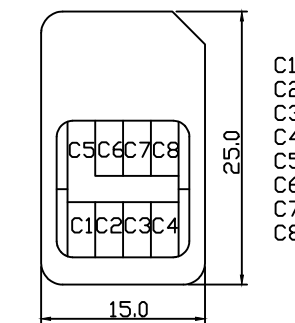
SIM CARD BOTTOM VIEW
