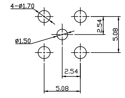
PCB Mounting Hole
