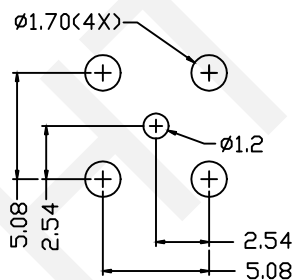
PCB MOUNTING HOLES
