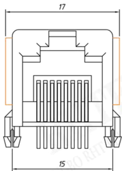
With Panel
