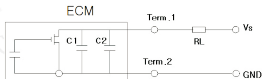
Schematic diagram VS=2V RL=2.2K
