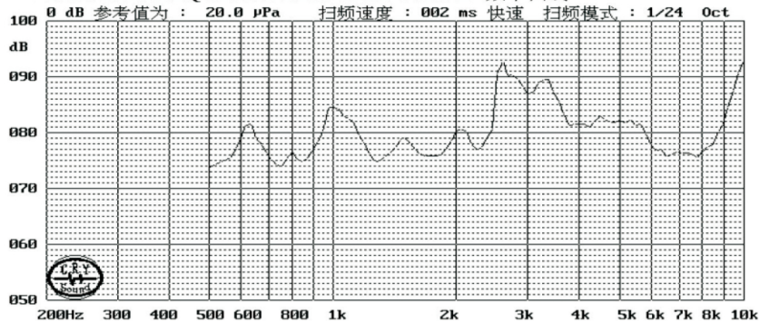
TYPICAL FREQUENCY RESPONSE CURVE 频率曲线
